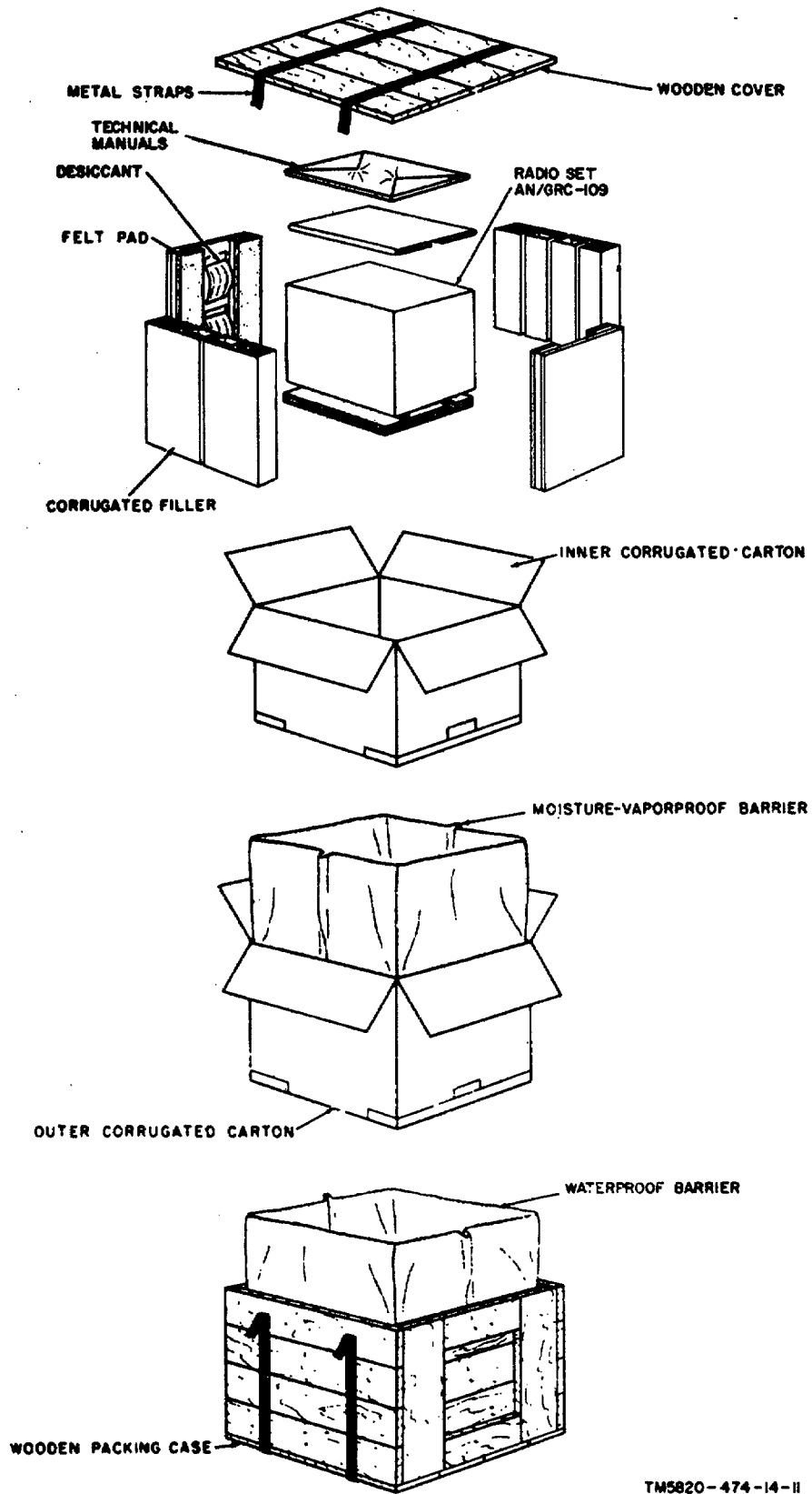
Figure 6. Typical packaging.
