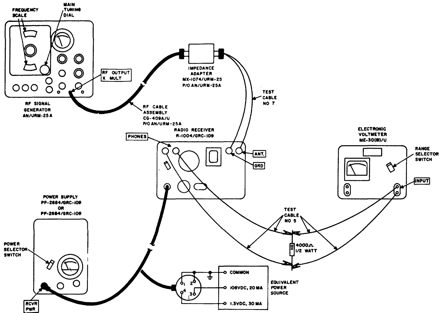
Figure 58. Receiver image rejection test.
