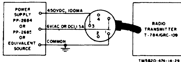
Figure 29. Test setup for troubleshooting transmitter.
