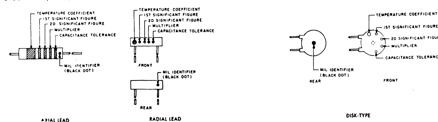
Figure 62. Color code marking for MIL-STD capacitors.
